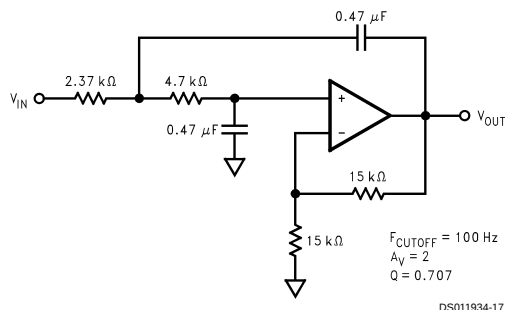
FIGURE 10. Low Pass Filter
