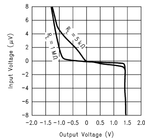
Input Voltage vs Output Voltage ( V_S = \pm 1.5 )
