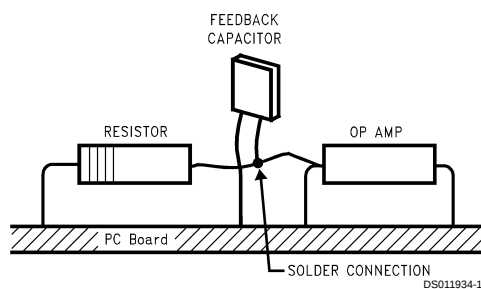
FIGURE 5. Air Wiring
