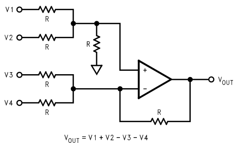
FIGURE 9. Adder/Subtractor Circuit
