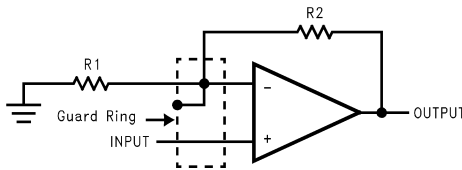
Non-Inverting Amplifier
